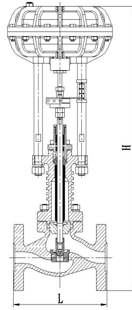
KP-28 with Bellows
