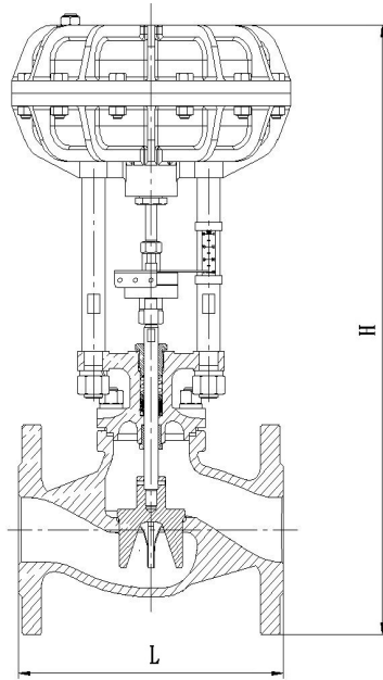
KP-28 without Bellows
