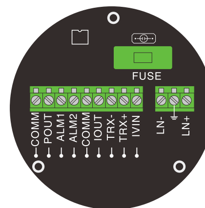
Terminal Configuration
