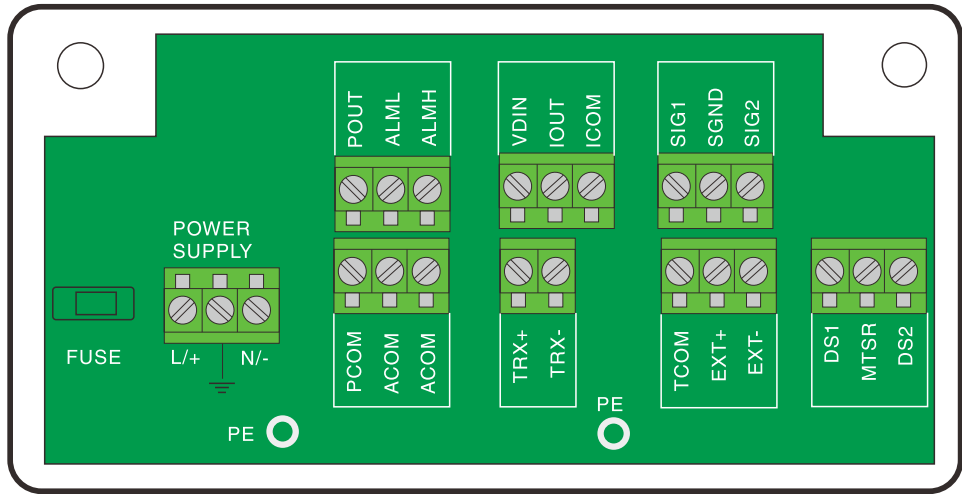
Terminal Configuration
