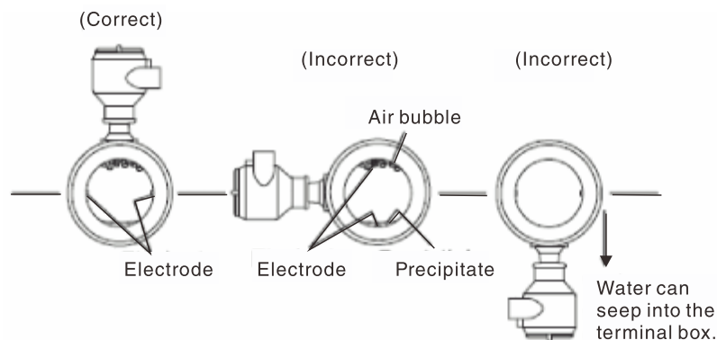
Mounting Orientation
